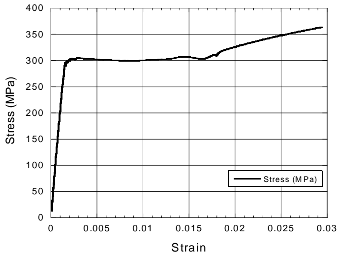
Figure 5. Stress-strain response of existing members
