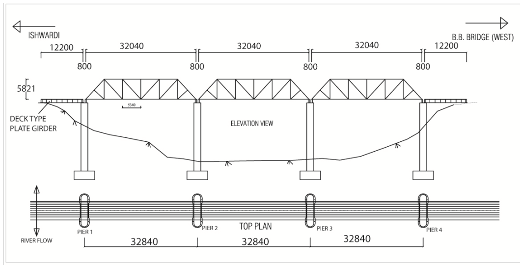
Figure 4. General dimensions of Boral Bridge and span arrangements
