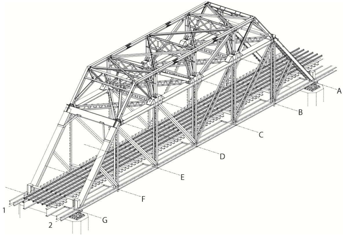
Figure 6. Post-survey reconstructed shop drawings and renovation plan for a typical span
